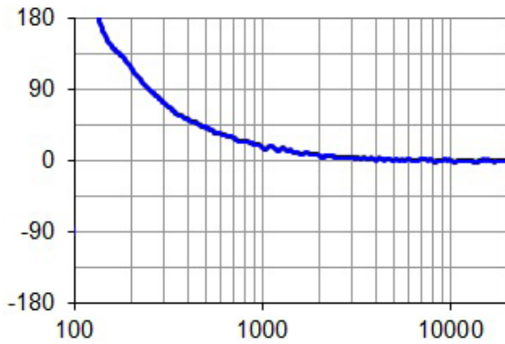
PHASE LINEARITY
